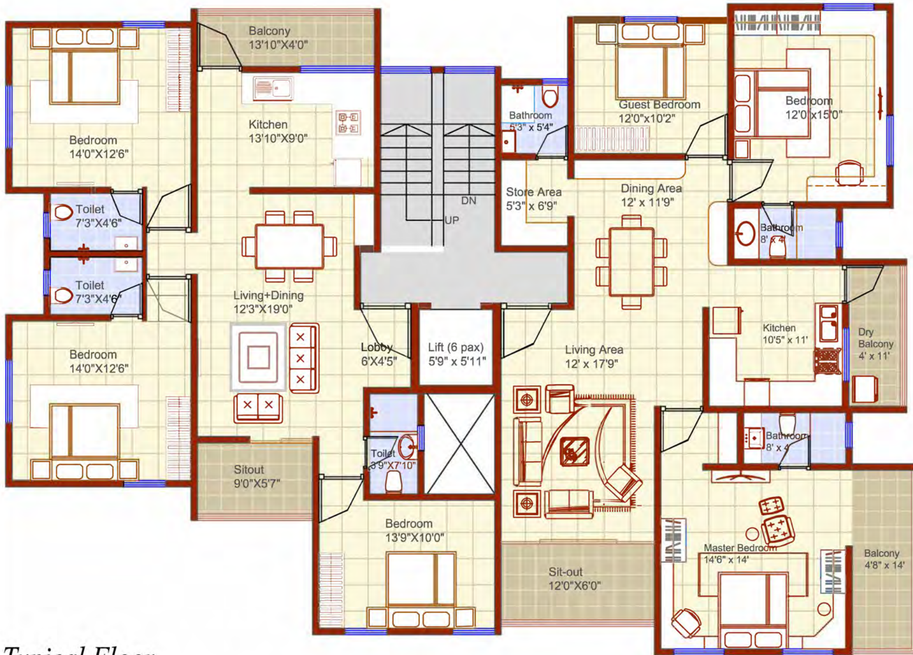
Typical Floor
